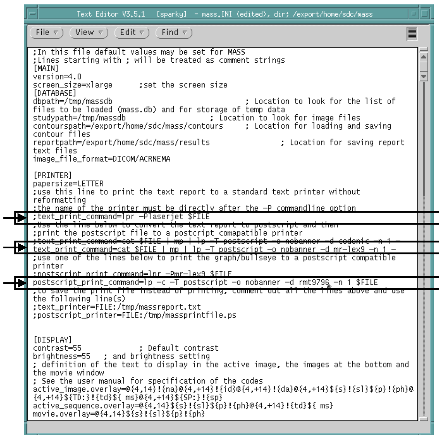
TEXT EDITOR WINDOW ILLUSTRATION 3-1
